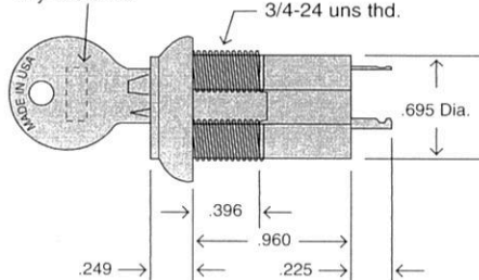
PC Mounting
